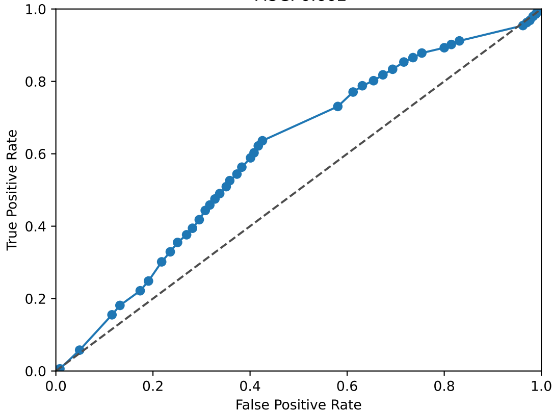
STAT2 ROC Curve AUC: 0.602
