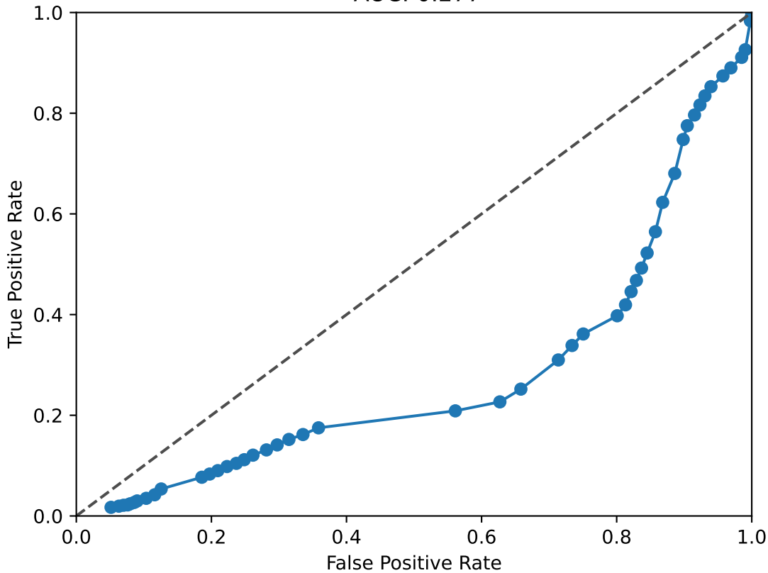
TCF7L1 ROC Curve AUC: 0.277
