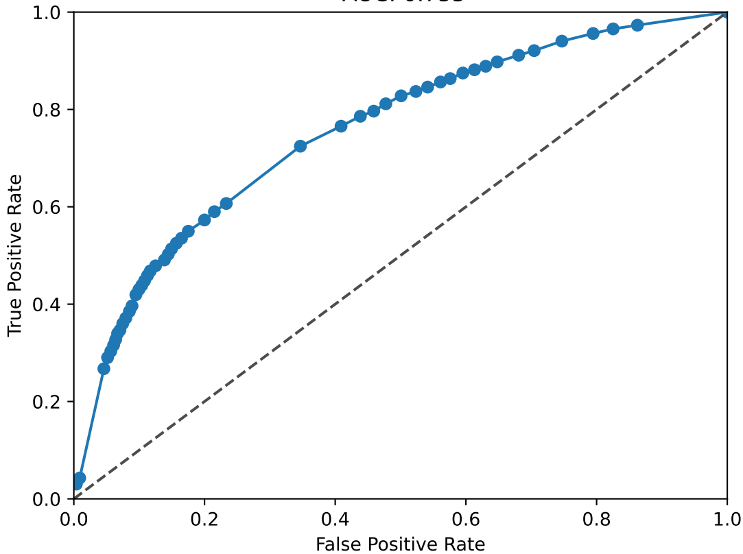
TEAD1 ROC Curve AUC: 0.755
