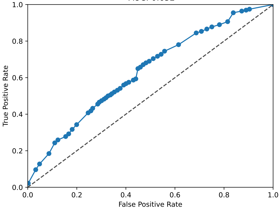
BACH1 ROC Curve AUC: 0.632
