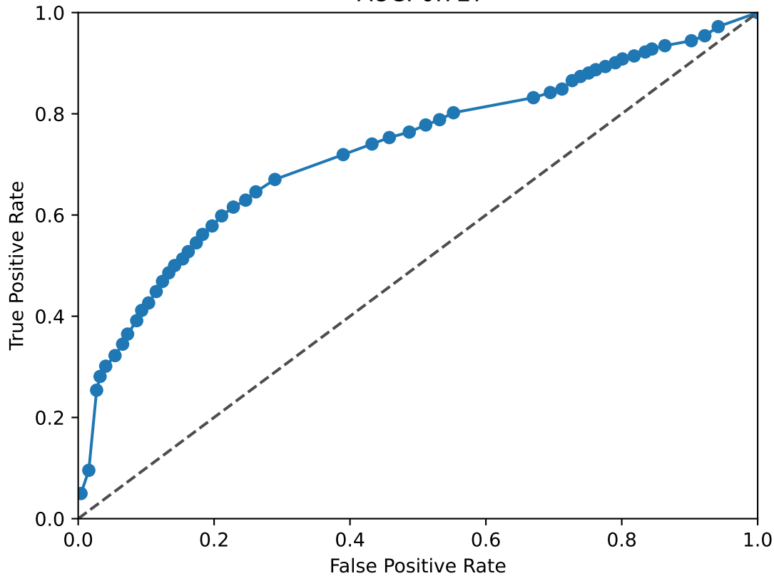
FOS ROC Curve AUC: 0.727
