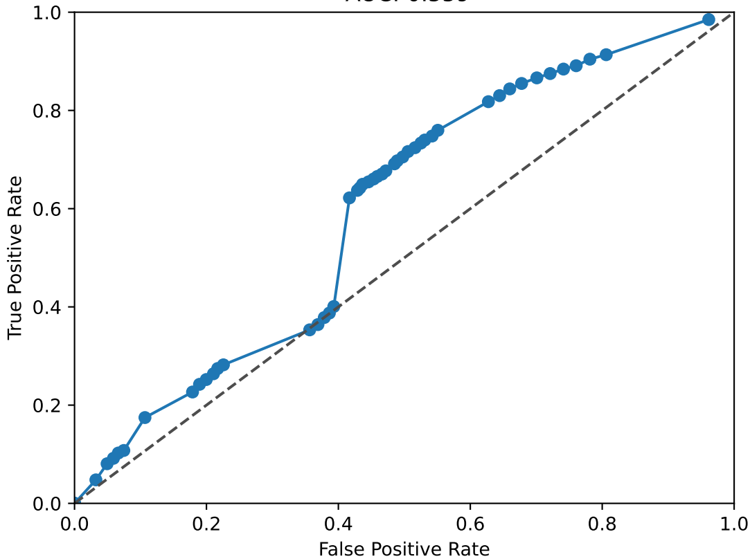
FOXO3 ROC Curve AUC: 0.559
