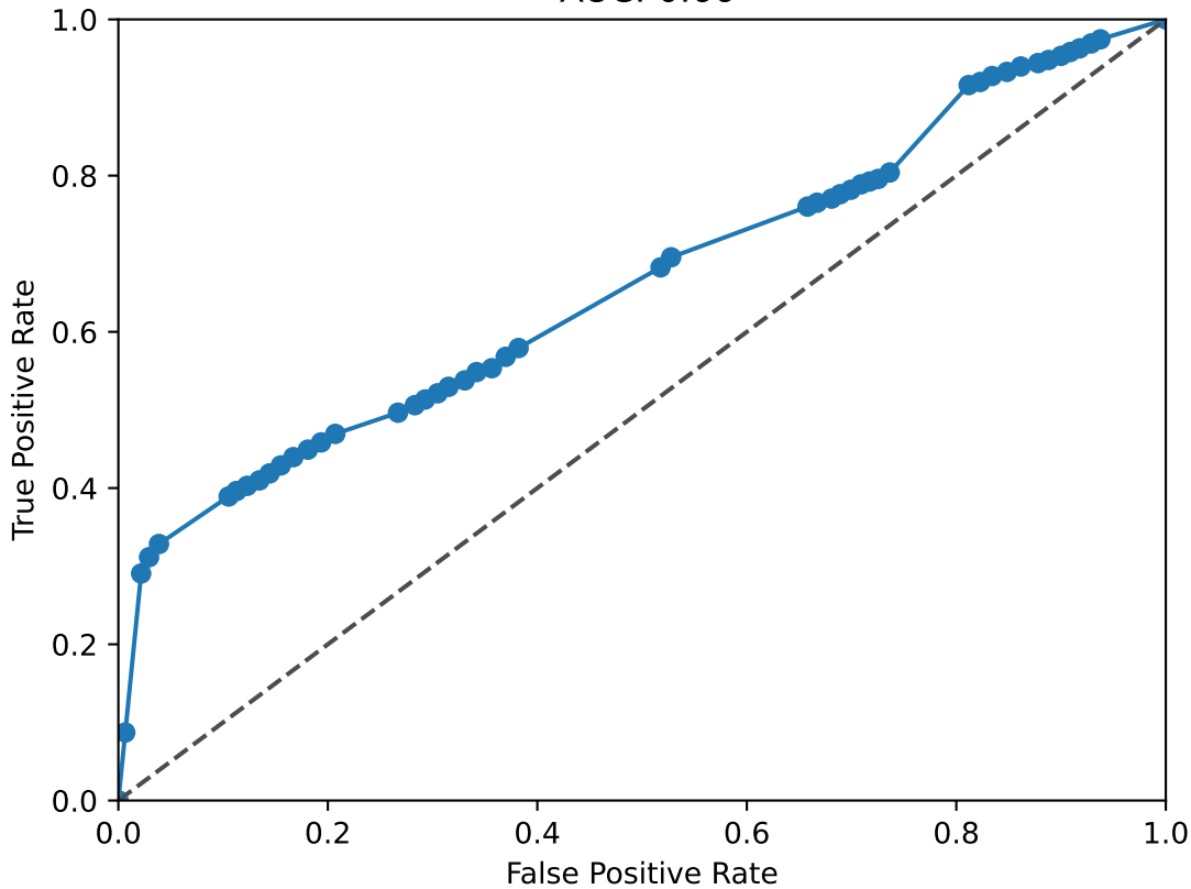
JUNB ROC Curve AUC: 0.66
