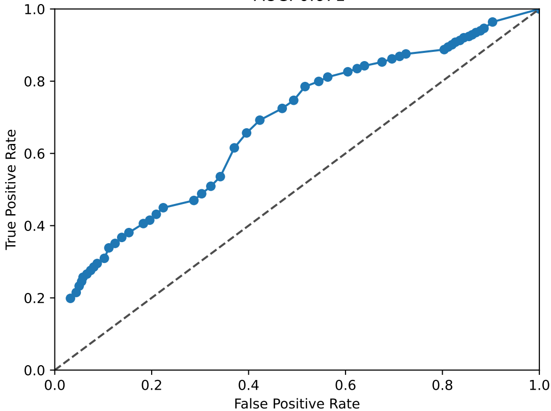
JUN ROC Curve AUC: 0.671
