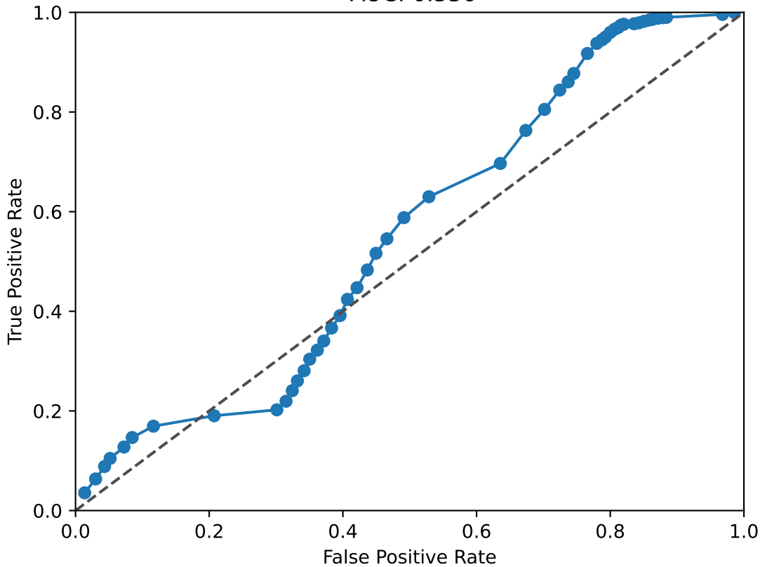
KMT2A ROC Curve AUC: 0.536
