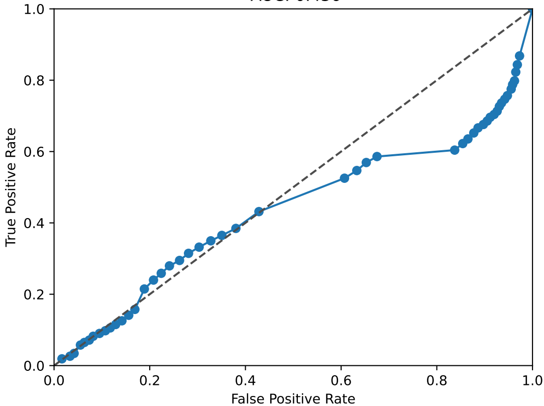
NFIB ROC Curve AUC: 0.436
