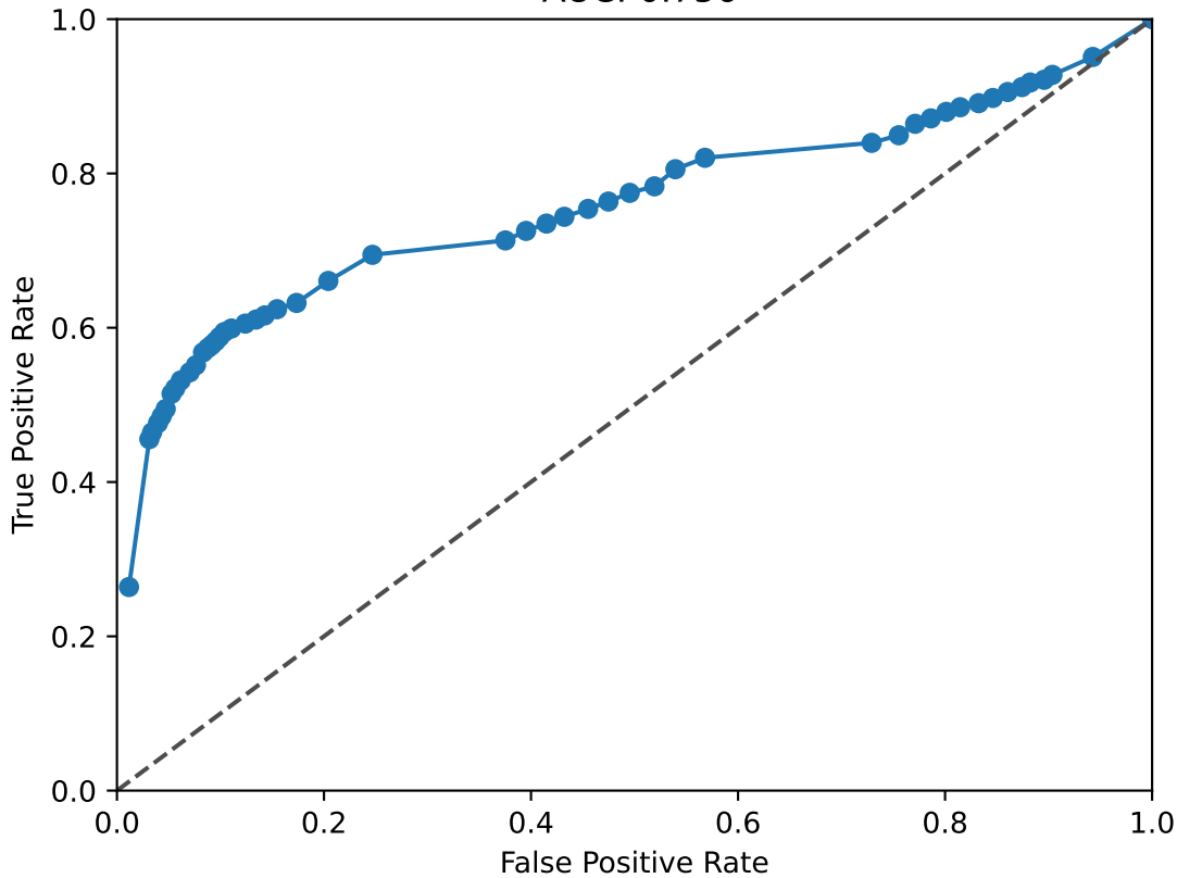
NFIX ROC Curve AUC: 0.756
