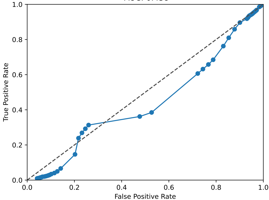
PBX1 ROC Curve AUC: 0.438
