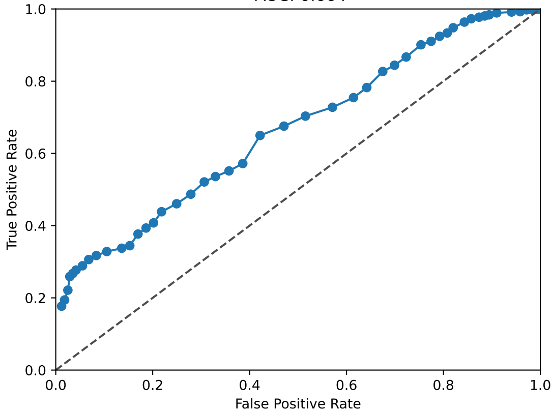
RUNX1 ROC Curve AUC: 0.664
