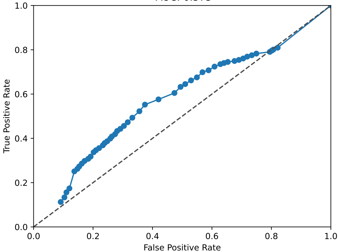
SIX1 ROC Curve AUC: 0.575
