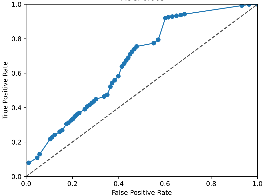
SOX11 ROC Curve AUC: 0.663
