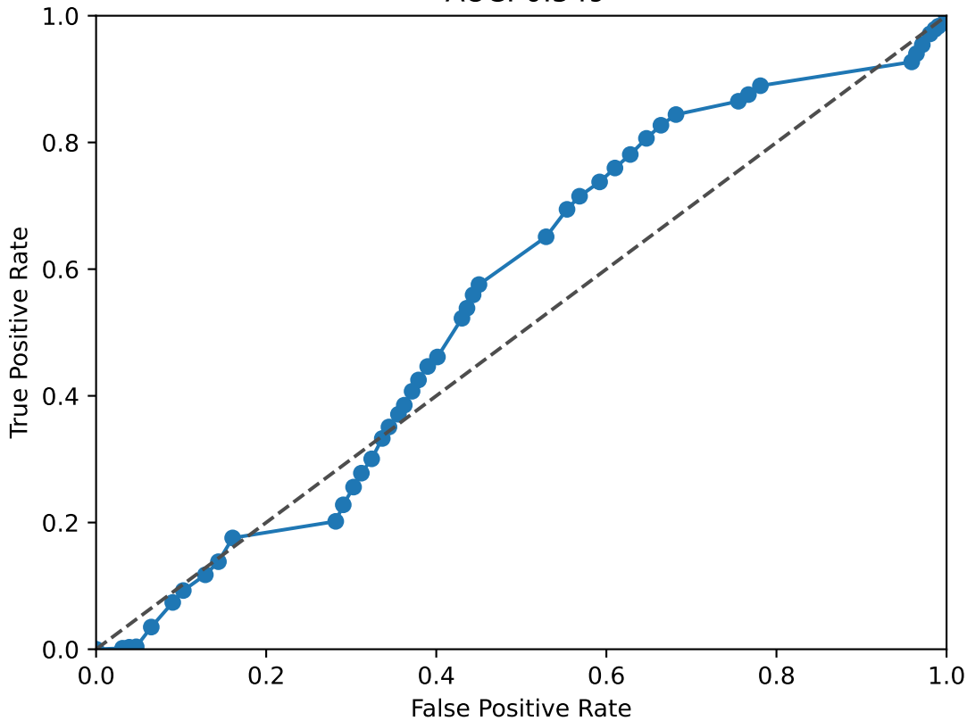
STAT2 ROC Curve AUC: 0.549
