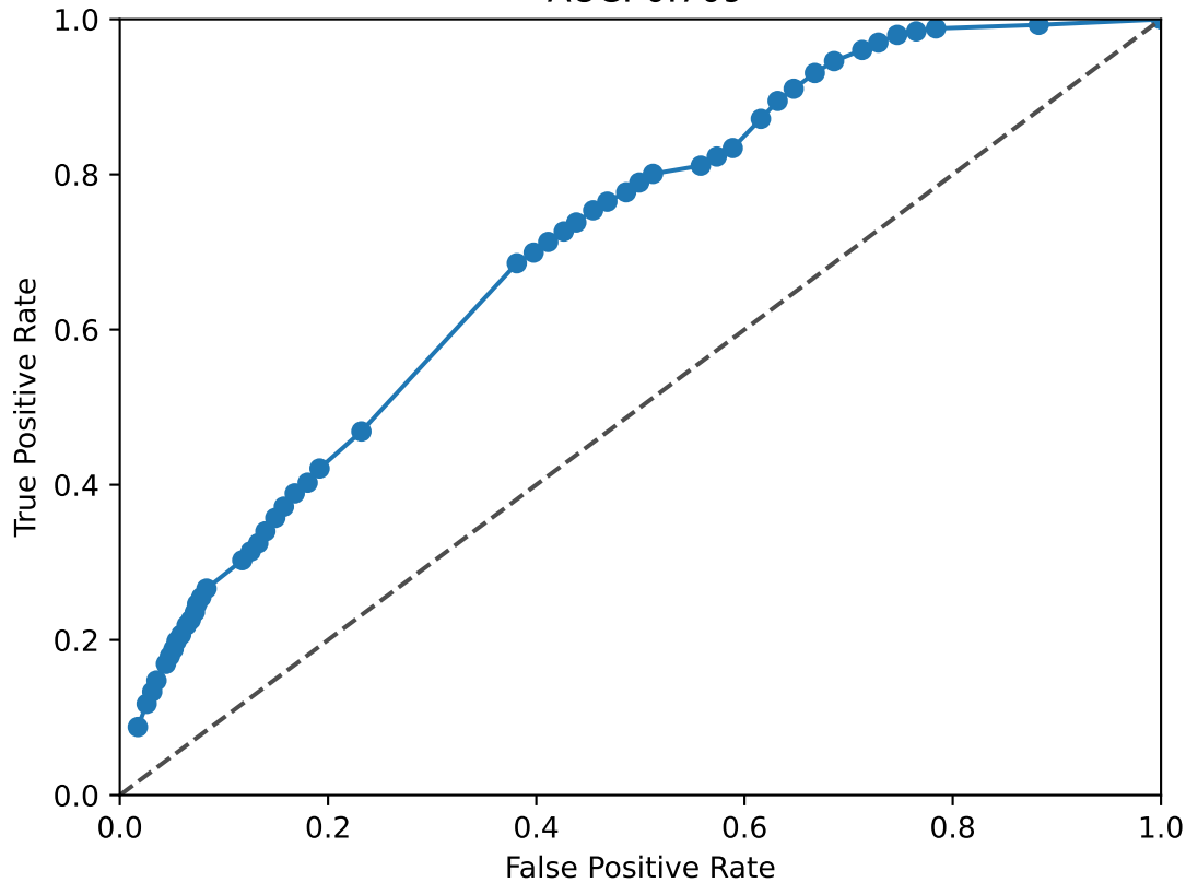
ASCL1 ROC Curve AUC: 0.709
