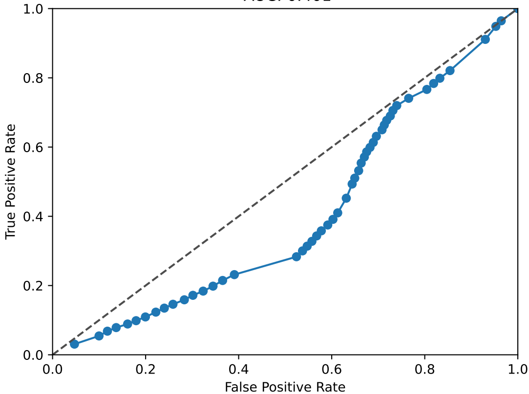
EPCAM ROC Curve AUC: 0.401
