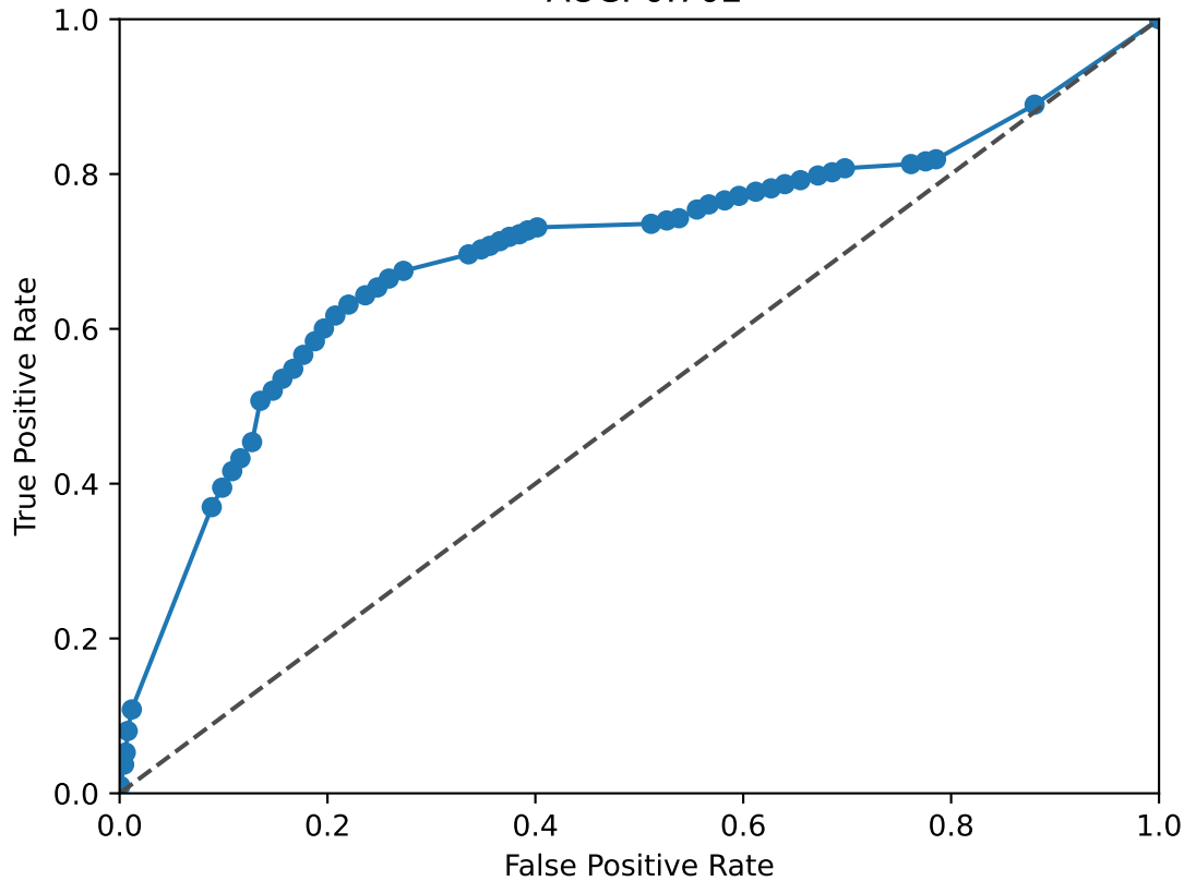
ETS1 ROC Curve AUC: 0.702
