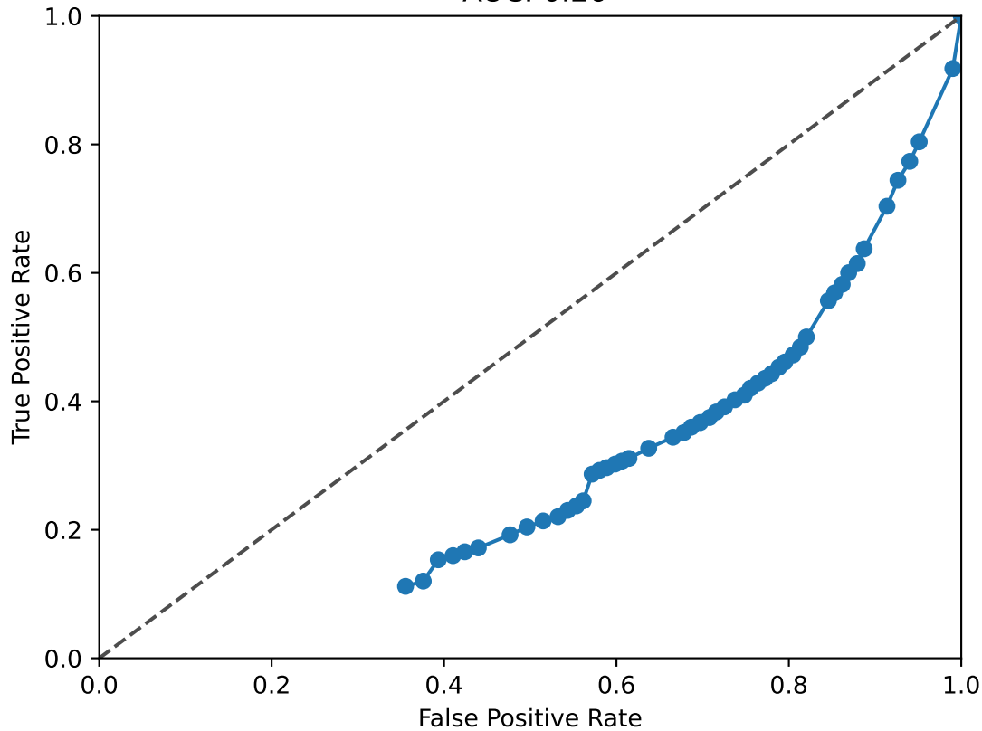
HES1 ROC Curve AUC: 0.26
