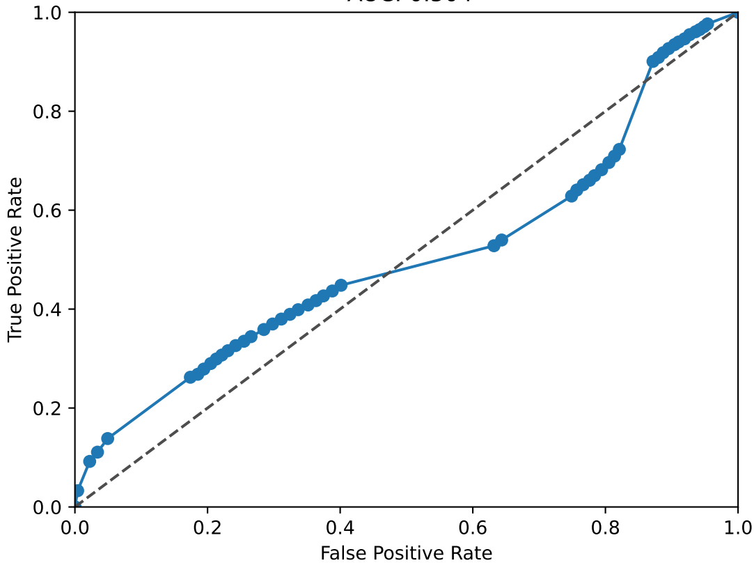
JUNB ROC Curve AUC: 0.504
