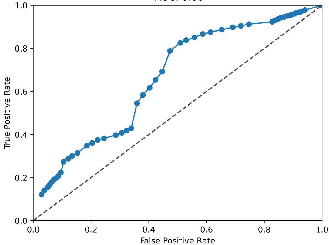
JUN ROC Curve AUC: 0.66
