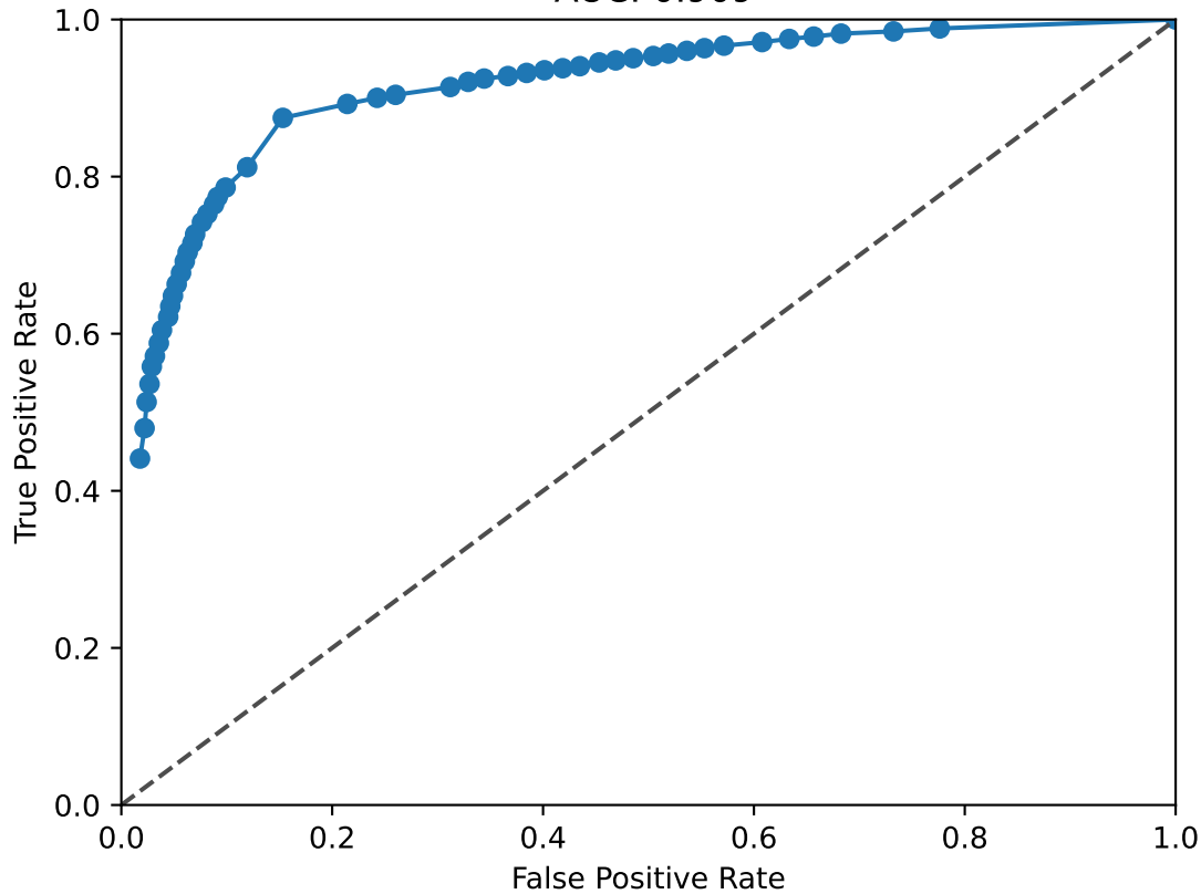
NCAM1 ROC Curve AUC: 0.909
