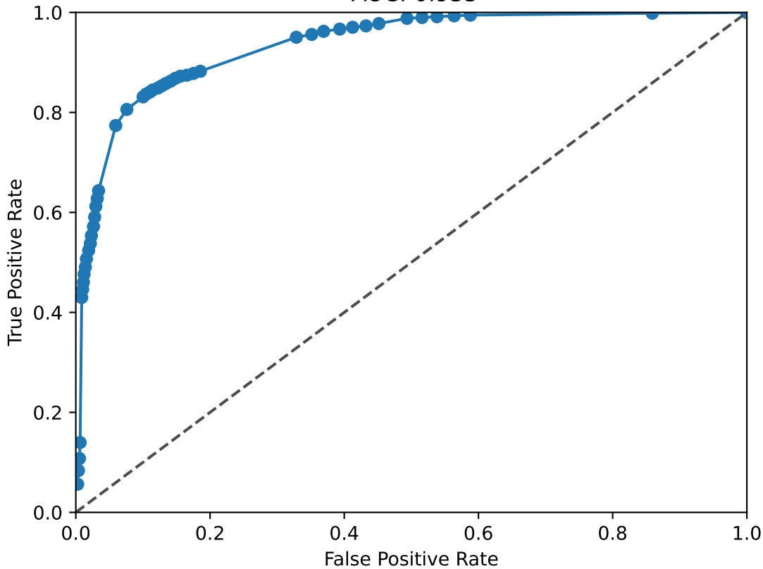
NFATC2 ROC Curve AUC: 0.935
