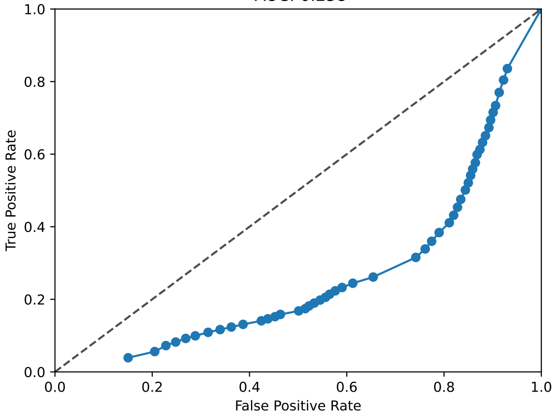
NFIB ROC Curve AUC: 0.258
