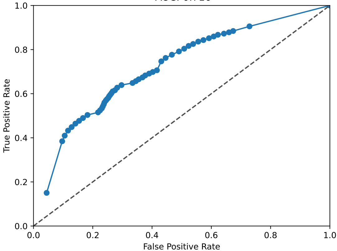
NFIX ROC Curve AUC: 0.716
