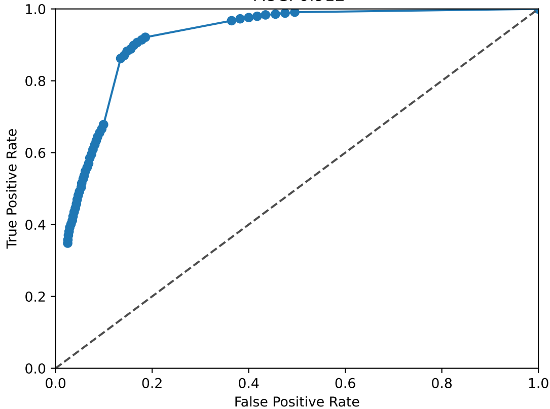
PROX1 ROC Curve AUC: 0.912
