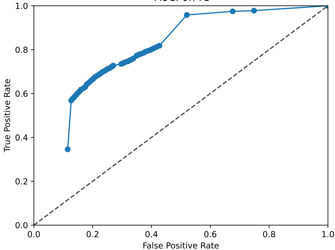
REST ROC Curve AUC: 0.773
