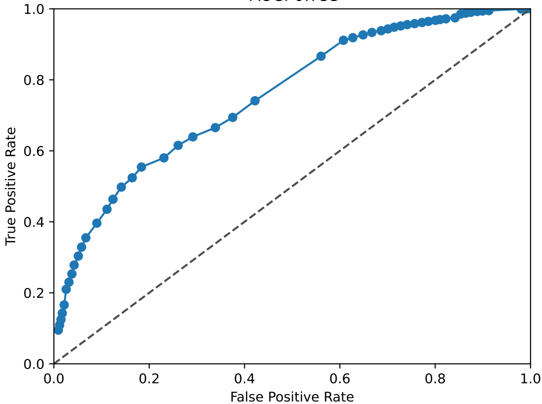
SIX4 ROC Curve AUC: 0.753
