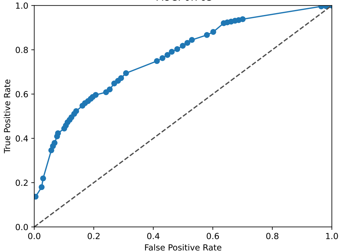
SOX11 ROC Curve AUC: 0.763
