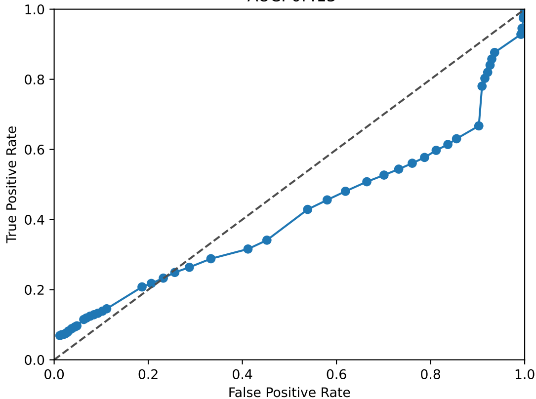
TCF7L1 ROC Curve AUC: 0.413
