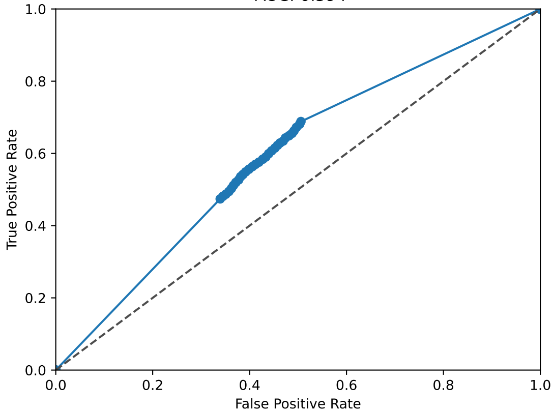
THR B ROC Curve AUC: 0.594
