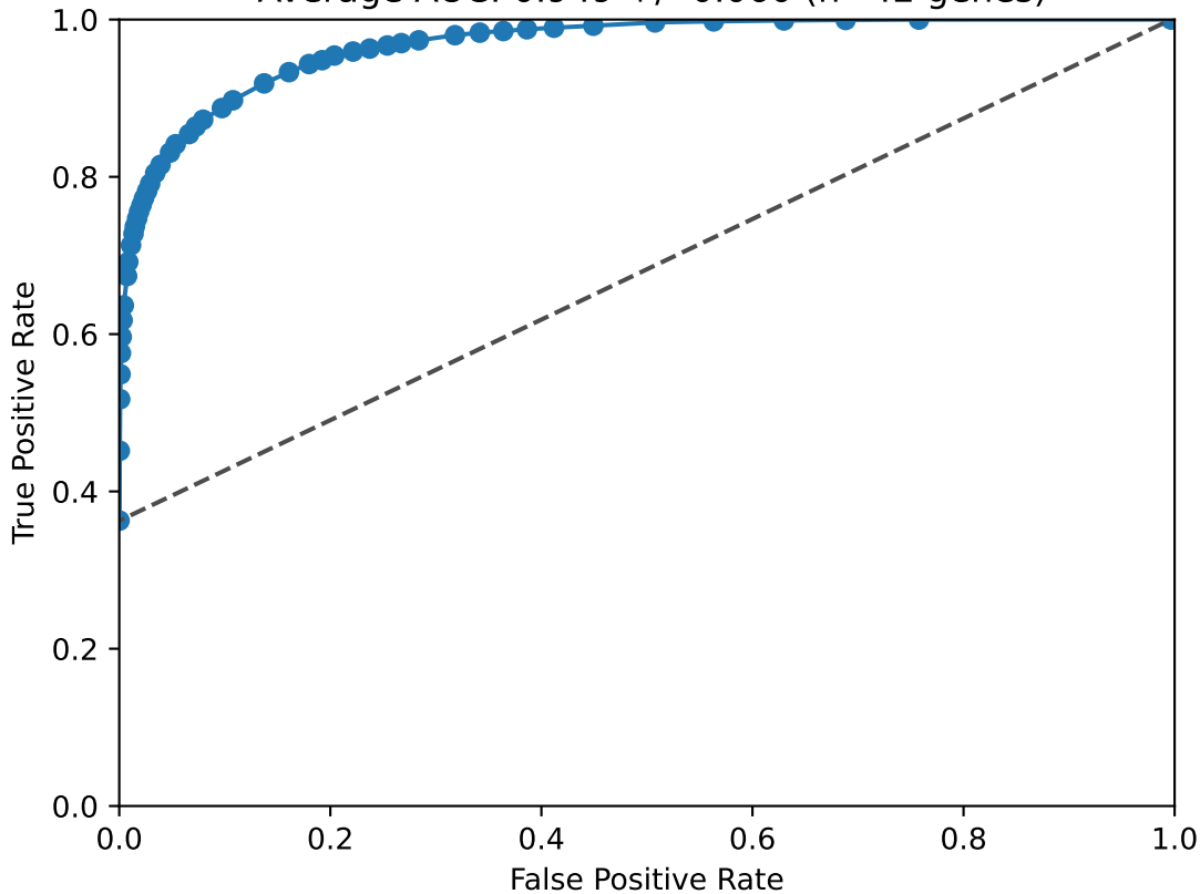
ROC Curve Data Average AUC: 0.949 \pm 0.060 (n=42 genes)
