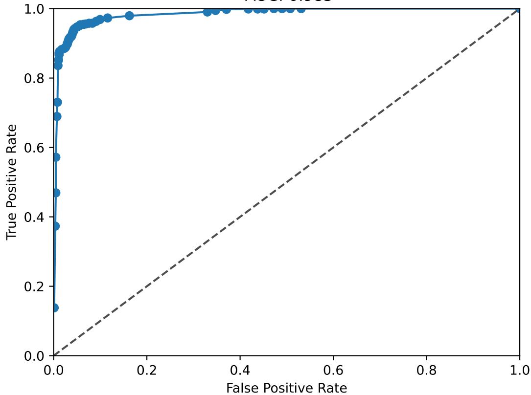
BACH1 ROC Curve AUC: 0.985
