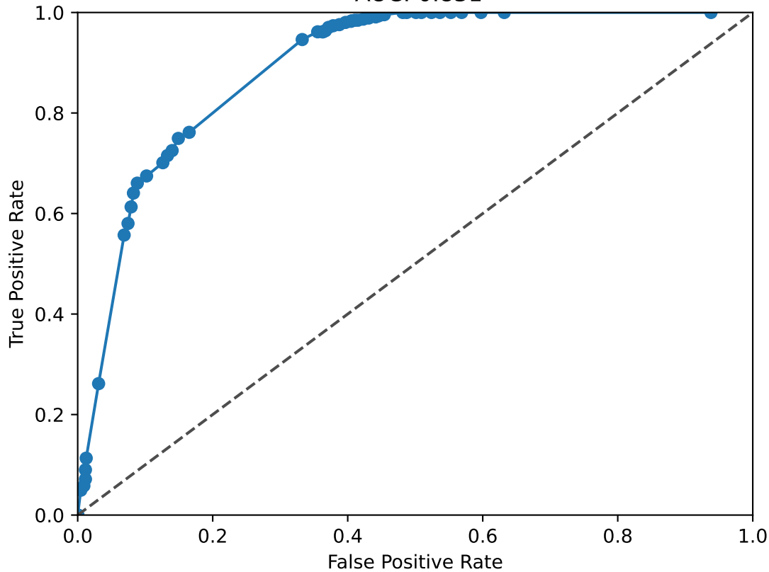
FOXO3 ROC Curve AUC: 0.831
