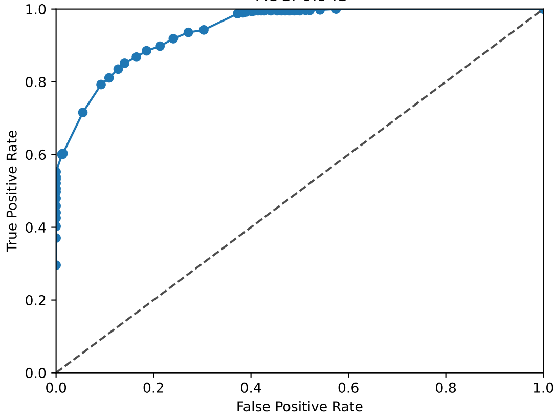
HES1 ROC Curve AUC: 0.943
