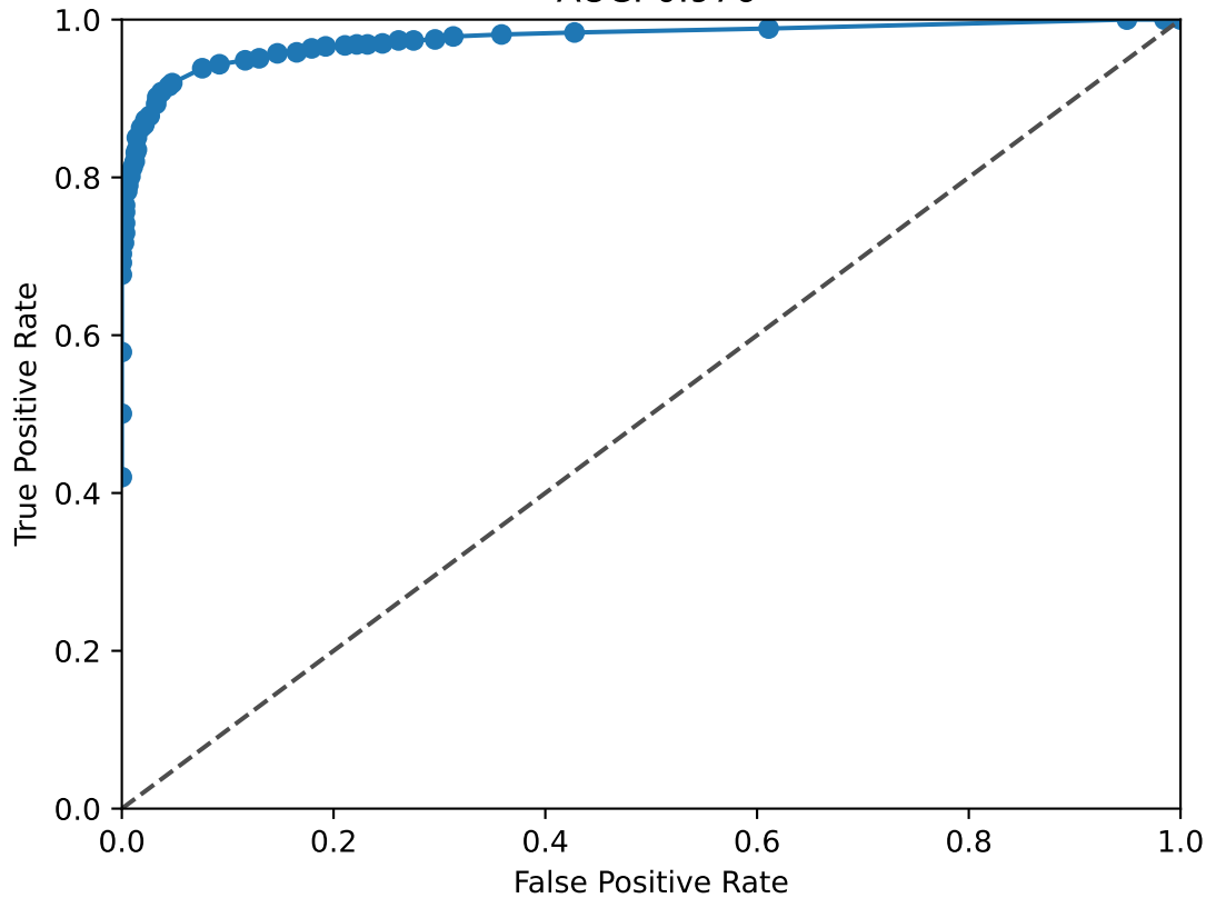
HSF2 ROC Curve AUC: 0.976
