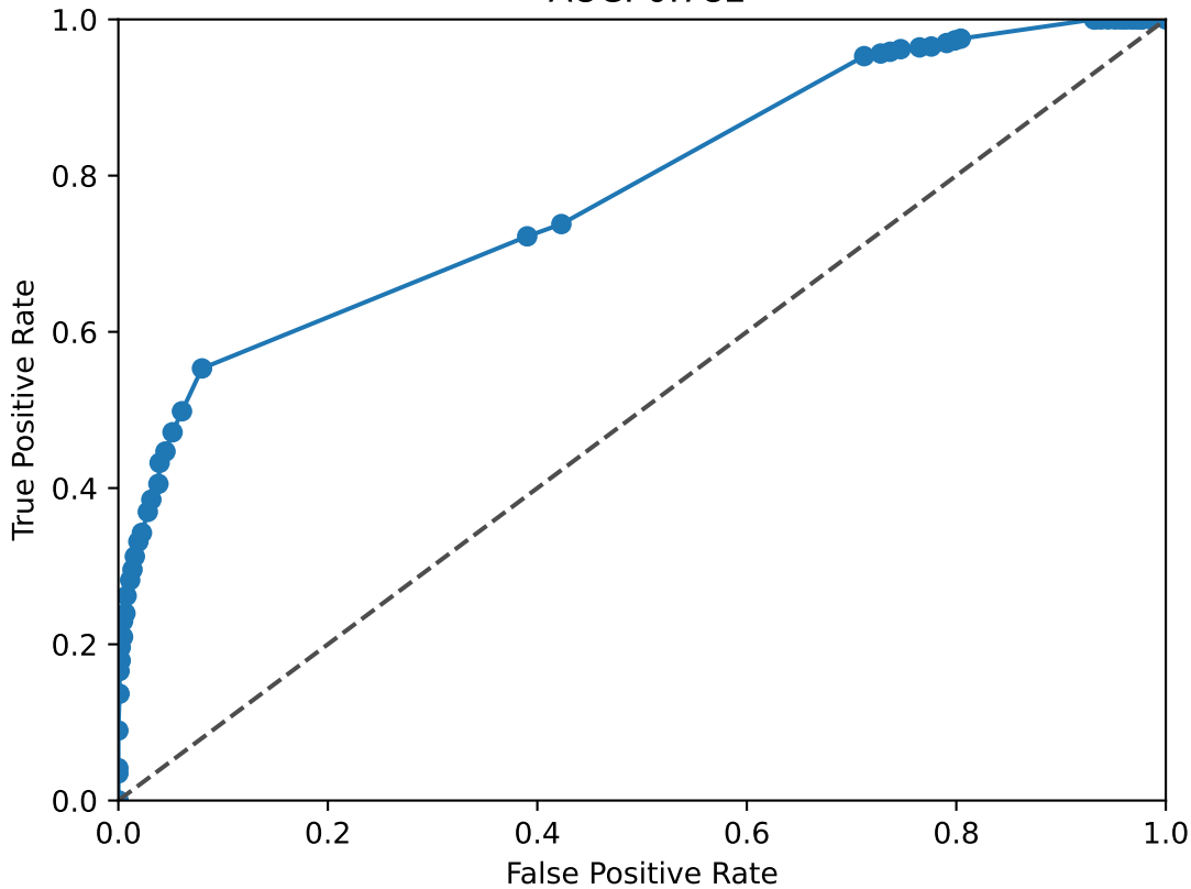
JUNB ROC Curve AUC: 0.782
