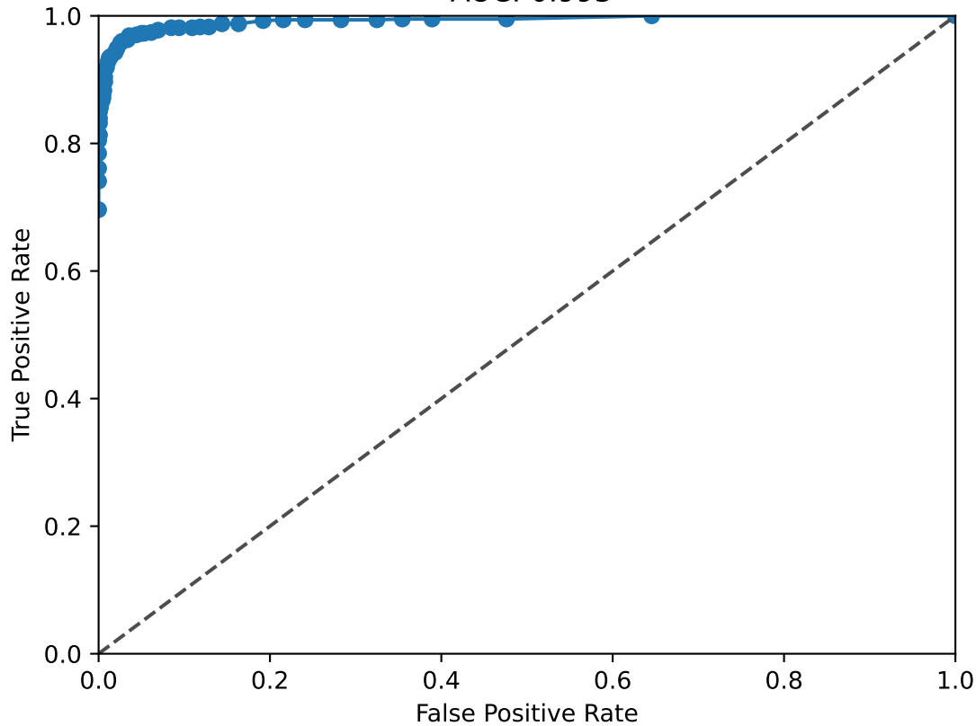
NCAM1 ROC Curve AUC: 0.993
