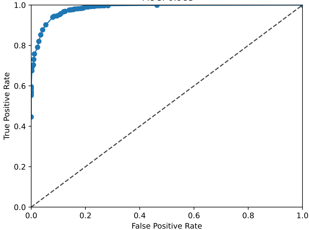
NFIX ROC Curve AUC: 0.983
