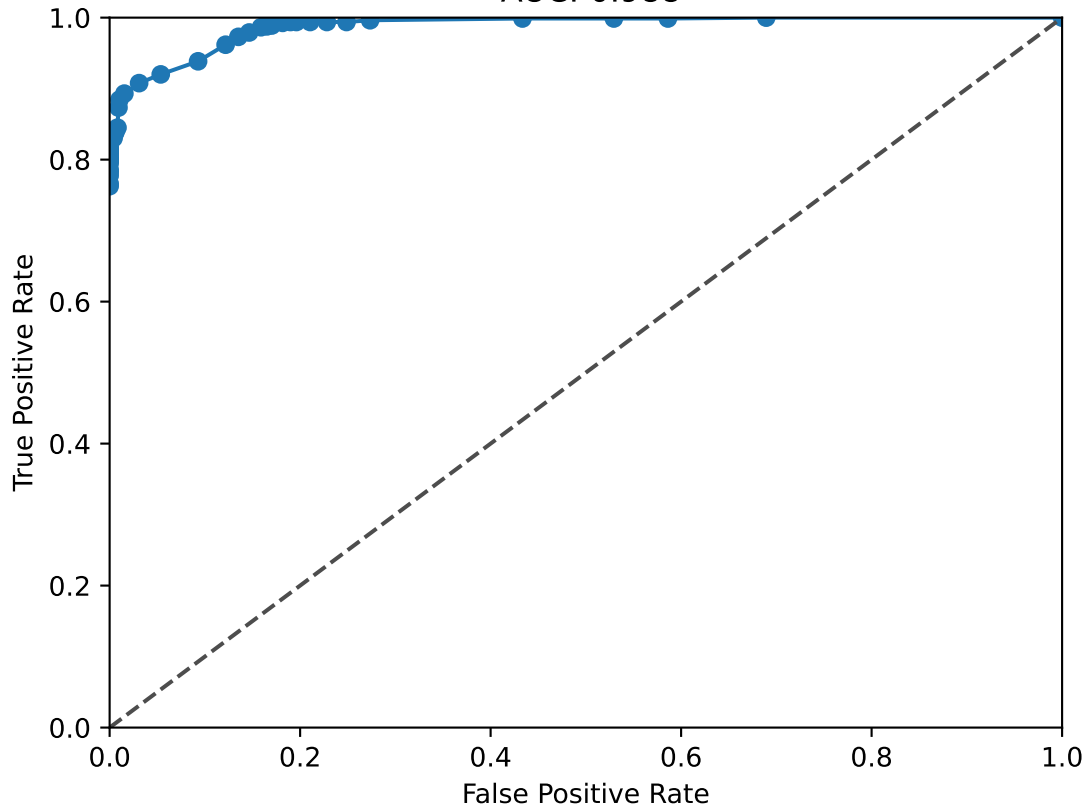
SIX1 ROC Curve AUC: 0.988
