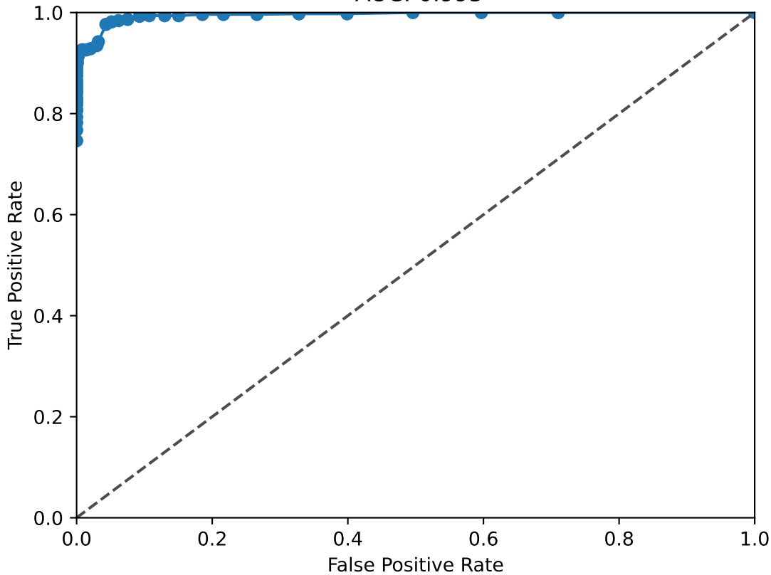
SIX4 ROC Curve AUC: 0.995
