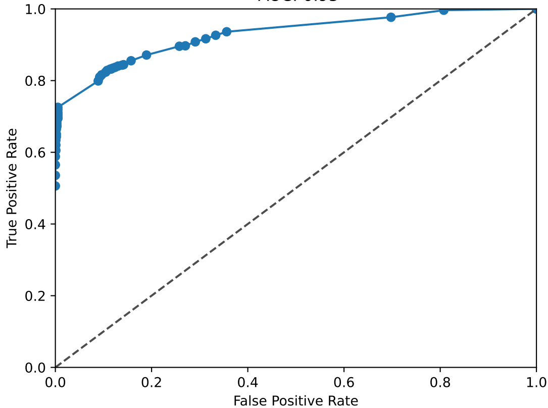
SOX11 ROC Curve AUC: 0.93
