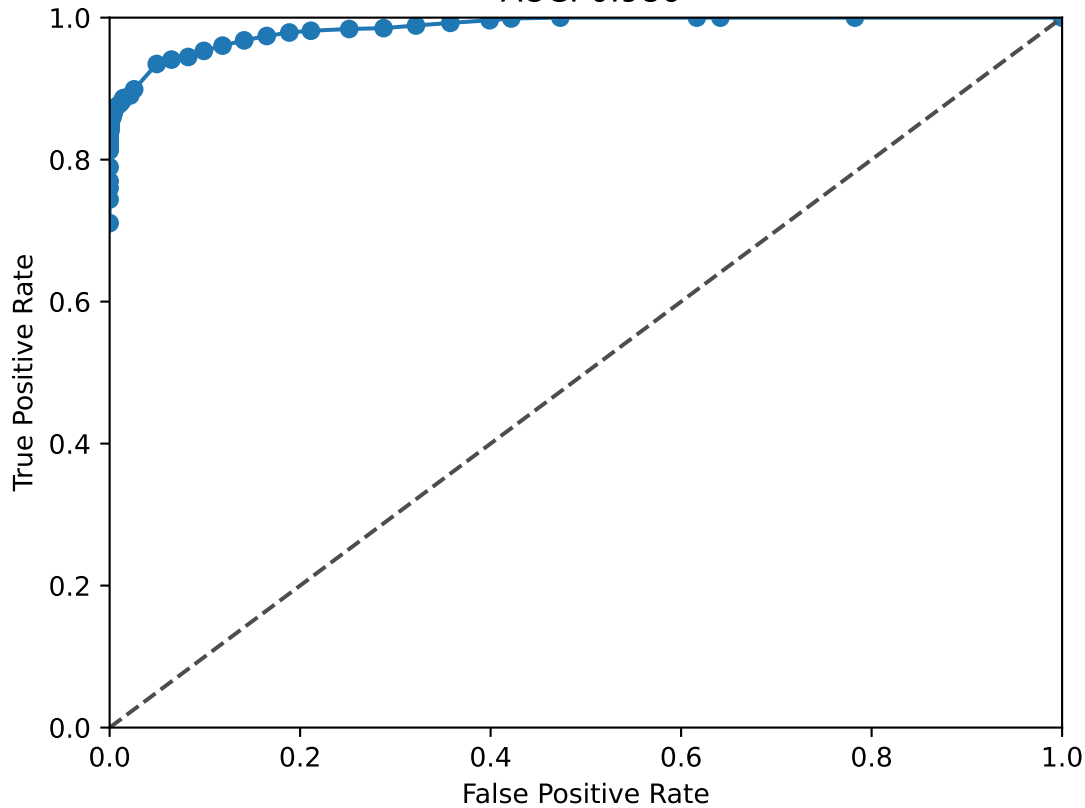
TBX15 ROC Curve AUC: 0.986
