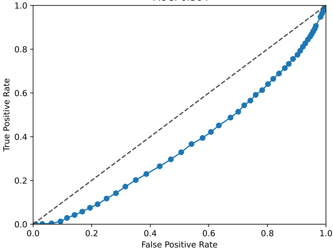
EPCAM ROC Curve AUC: 0.364
