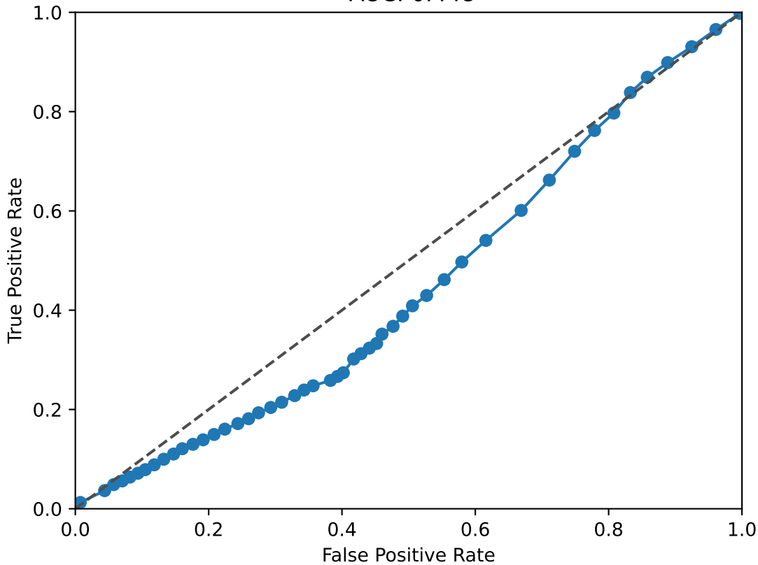
ICAM1 ROC Curve AUC: 0.448
