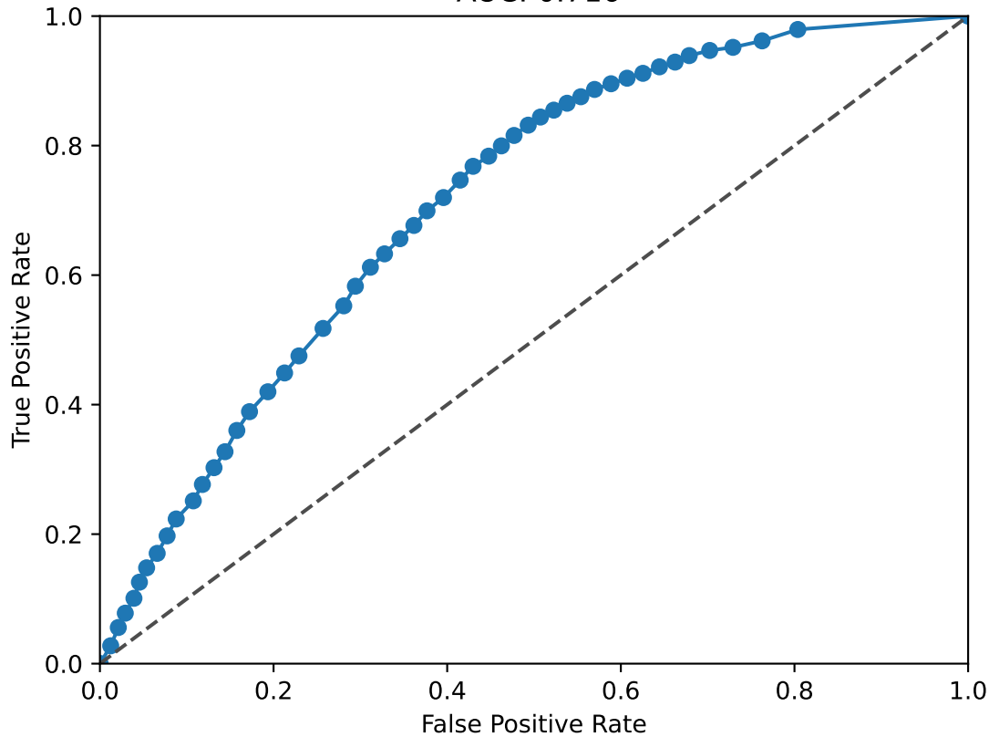
NCAM1 ROC Curve AUC: 0.716
