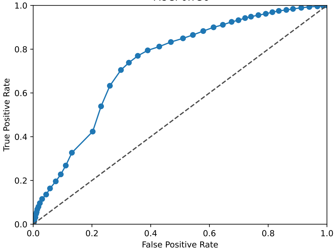
NFIA ROC Curve AUC: 0.736
