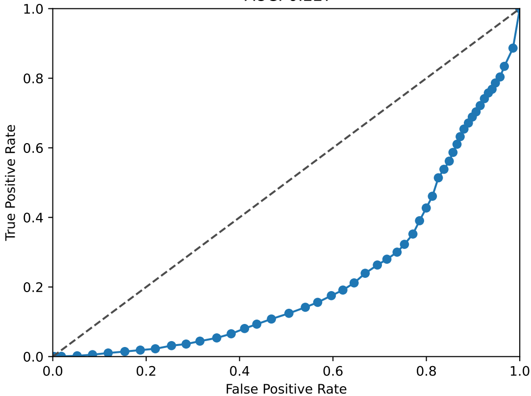
NFIB ROC Curve AUC: 0.227
