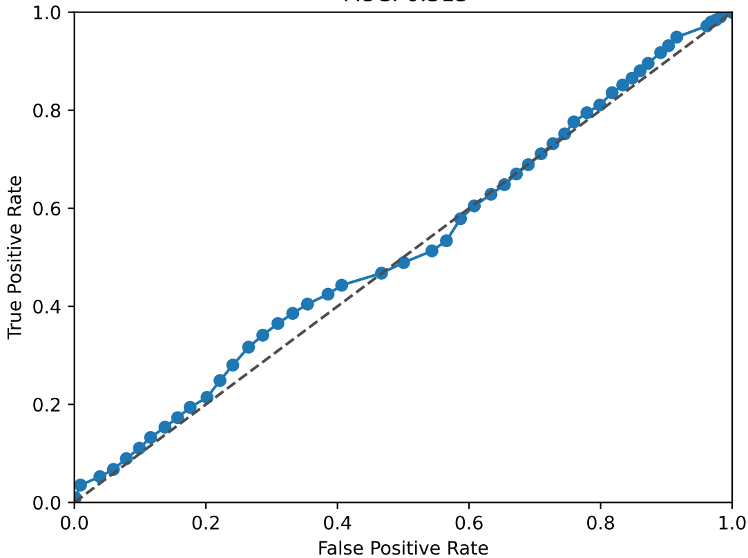
PKNOX2 ROC Curve AUC: 0.515
